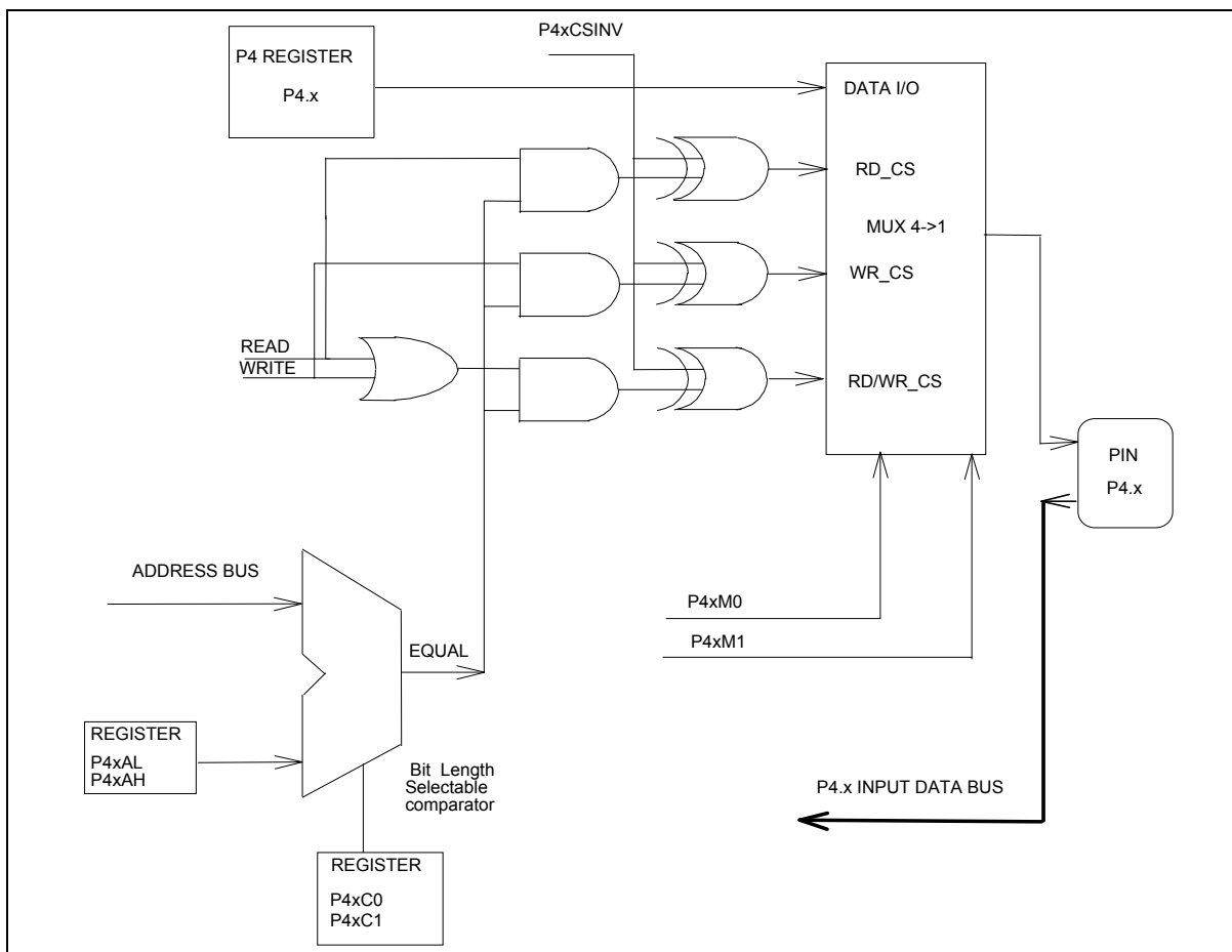
Figure 22-1: Port 4 Structure Diagram
