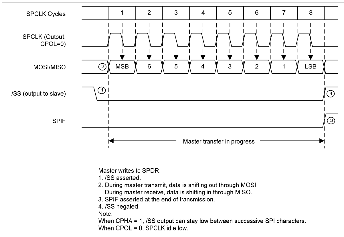
Figure 18-4: Master Mode Transmission (CPOL = 0, CPHA = 1)
